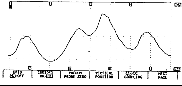
◎第二缸汽門黏滯
