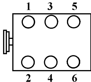
(C) 6缸、DIS
