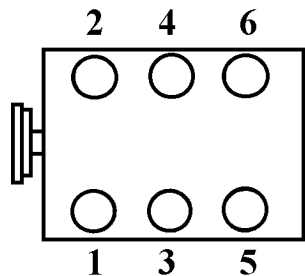
(A) 6缸、C3I
